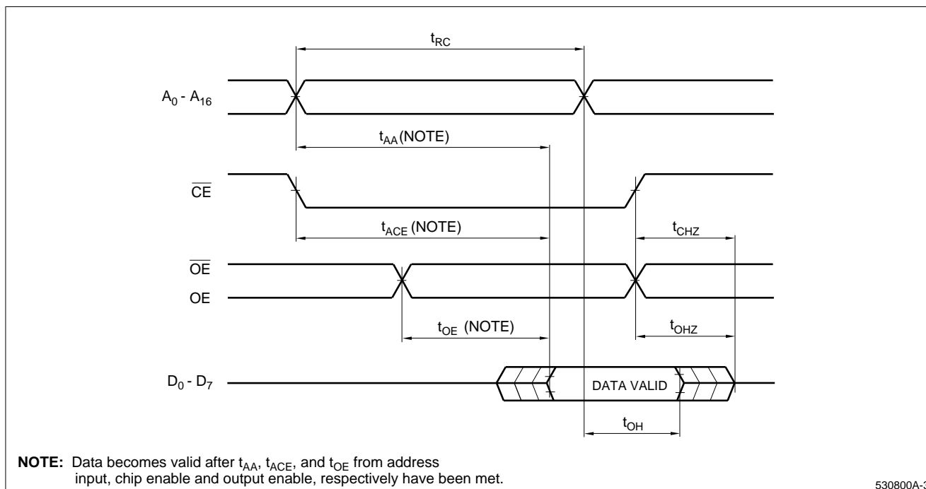
Figure 4. Timing Diagram
